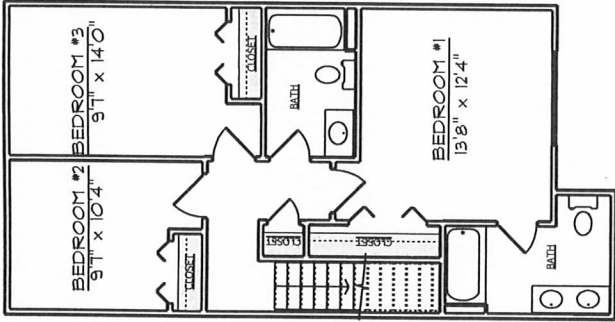
"Dover" 2nd Floor Plan
