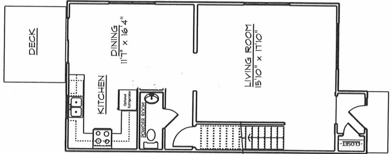
"Brandywine" 1st Floor Plan
