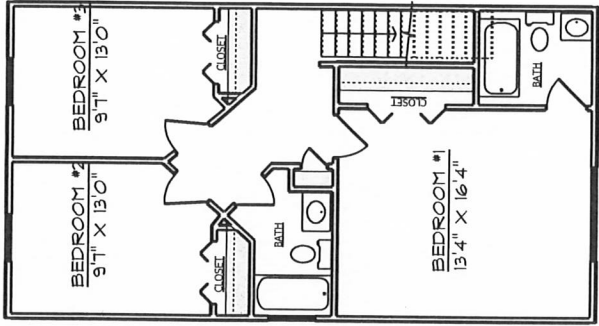
"Georgetown" 2nd Floor Plan
